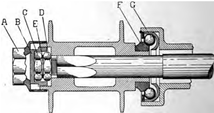
FIG. 388.—One Form of Driving Axle Using Ball Bearings. The hub is secured in place by the nuts and binders shown at A, B, C, D, E. At its inner extremity it carries a cone, F, which works on the ball race, G. The hub is thus suspended on the ball race, which also acts to neutralize end thrusts.
